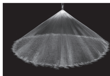
Full Cone 120° (W)
